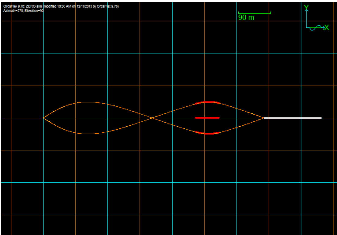
Figure 2. Examples of out-of-plane mode shapes.
