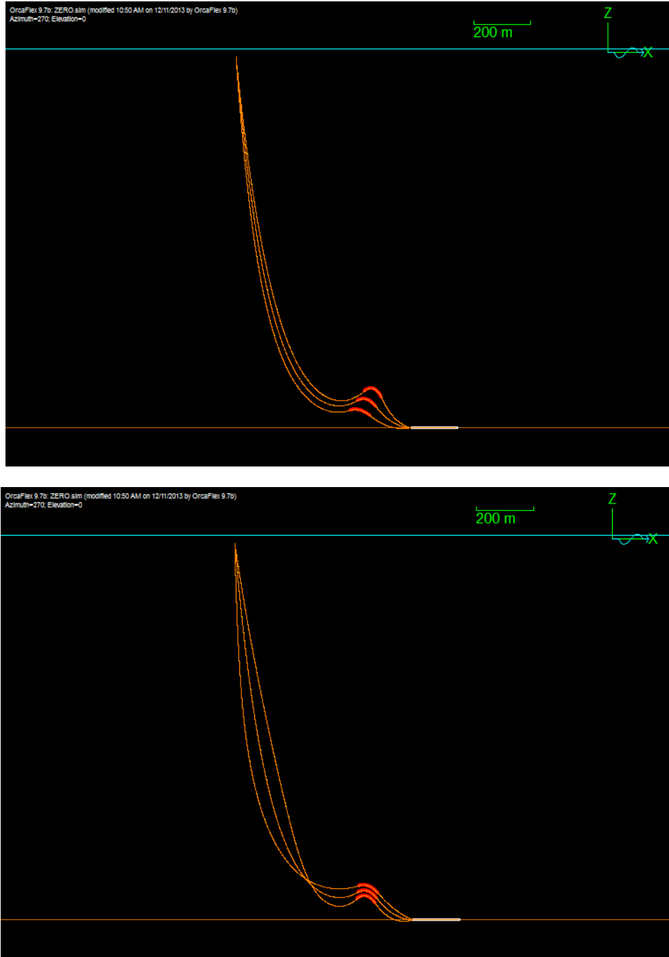
Figure 1. Examples of in-plane mode shapes.
